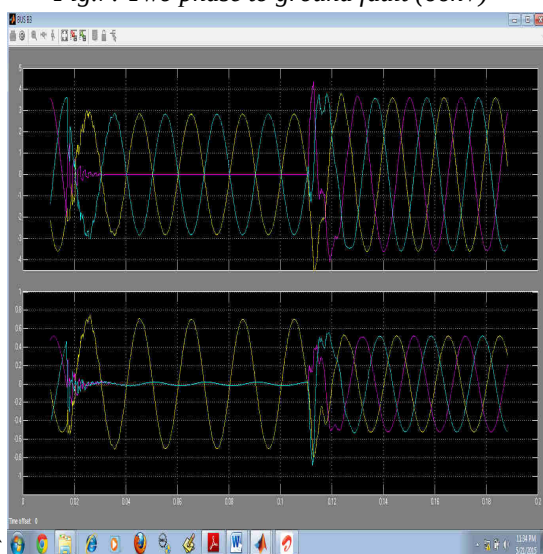
Fig.8: Two phase to ground fault (132kV)
